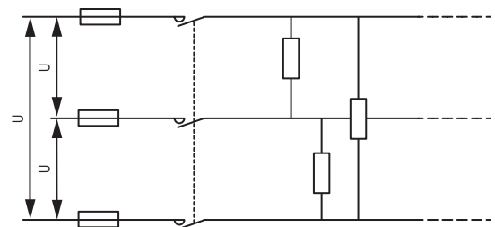
Three-phase (AC-1, AC-7a)
